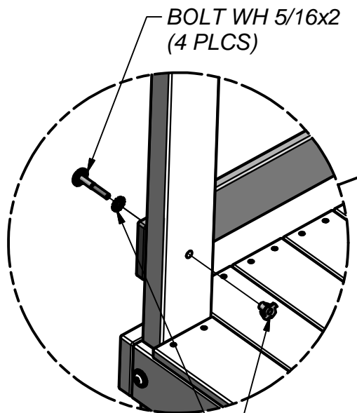
WASHER LOCK EXT 8x19 (4 PLCS) T-NUT 5/16 (4 PLCS)
