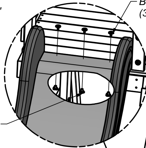
T-NUT 5/16 (3 PLCS)
